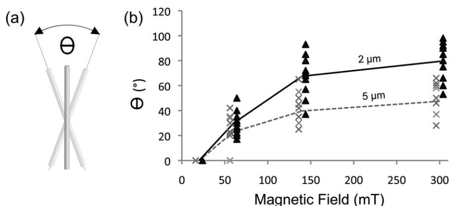
FIGURE 3. Movement quantification of magnetic nanorods in a live cell. (a) Definition of the total angular displacement \theta for an individual nanorod in response to a single revolution of the magnetic field (b) Total angular displacements of 2- \mu\text{m} (black) and 5- \mu\text{m} (gray) nanorods versus magnetic field intensity.
