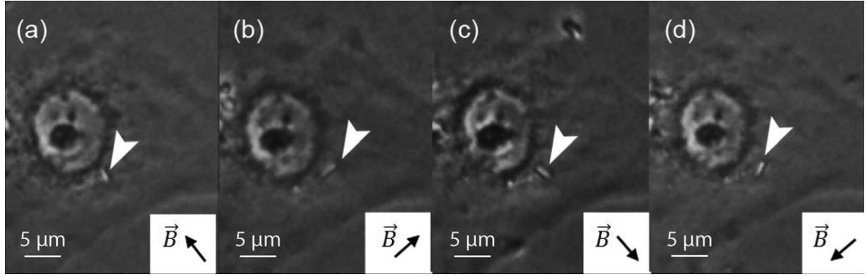
FIGURE 6. Complete rotation of a 2- \mu\text{m} nanorod following the external magnetic field orientation. (a) to (d) correspond to the magnetic field direction \vec{B} indicated.
